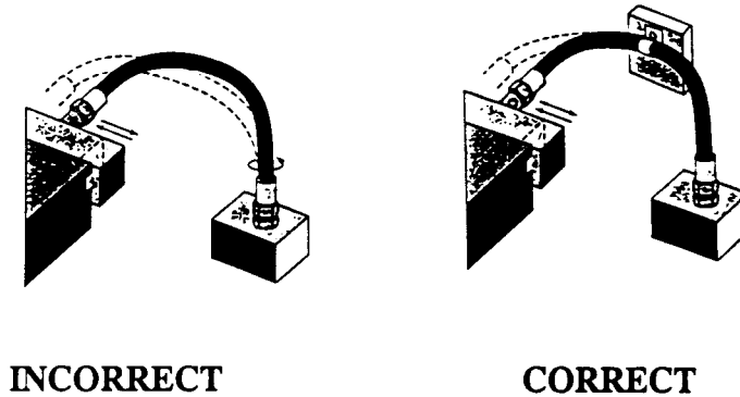
FIGURE 7—PREVENT HOSE BENDING IN MORE THAN ONE PLANE
