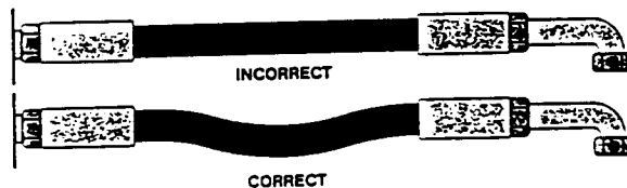
FIGURE 4—HOSE AND MACHINE TOLERANCES
